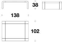
CTR (13) COFFEE TABLE / COCKTAIL TABLE 138x102x38H.cm 54 1/3x40x15H."
