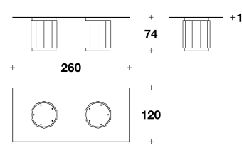
RTB (28V) TAVOLO / TABLE 260x120x74H. - THK.1 cm 102 1/3x47 1/3x29H. - THK.6/16 "
