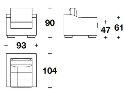
SHT (POL) POLTRONA / ARMCHAIR 93x104x90H. - H.A.61 - H.S.47 cm 36 2/3x41x35 1/3H. - H.A.24 - H.S.18 2/4 "
