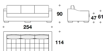
SHT (D3) DIVANO 3 POSTI / 3 SEATER SOFA 254x114x90H. - H.A.61 - H.S.47 cm 100x45x35 1/3H. - H.A.24 - H.S.18 2/4 "
