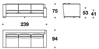
AFPYCA3BRD Height: 29 2/3" / 75 CM Width: 94" / 239 CM Depth: 37" / 94 CM Weight: 397 lbs / 180 kg
