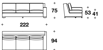
AFPYCE3S Height: 29 2/3" / 75 CM Width: 87 1/3" / 222 CM Depth: 37" / 94 CM Weight: 373 lbs / 169 kg
