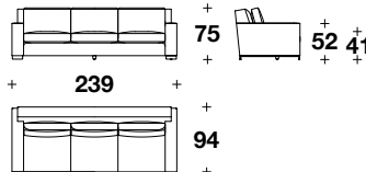
AFPYCD3 Height: 29 2/3" / 75 CM Width: 94" / 239 CM Depth: 37" / 94 CM Weight: 240 lbs / 109 kg
