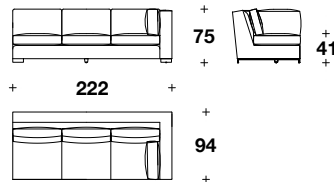
AFPYCA3D Height: 29 2/3" / 75 CM Width: 87 1/3" / 222 CM Depth: 37" / 94 CM Weight: 373 lbs / 169 kg
