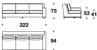
AFPYCE3D Height: 29 2/3" / 75 CM Width: 87 1/3" / 222 CM Depth: 37" / 94 CM Weight: 373 lbs / 169 kg
