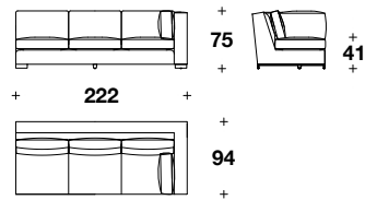
AFPYCA3S Height: 29 2/3" / 75 CM Width: 87 1/3" / 222 CM Depth: 37" / 94 CM Weight: 373 lbs / 169 kg
