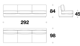
DSM (E3C) ELEMENTO CENTRALE 3 POSTI / 3 SEATER CENTRAL ELEMENT 292x98x84H. - H.S.45 cm 115x38 2/3x33H. - H.S.17 3/4 "
